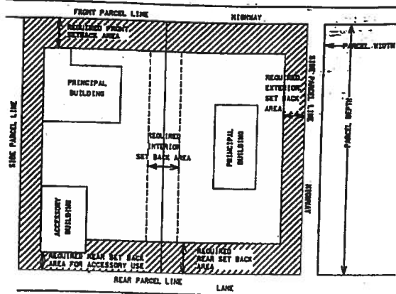
Diagram No. 2 SETBACK/HEIGHT DEFINITIONS
