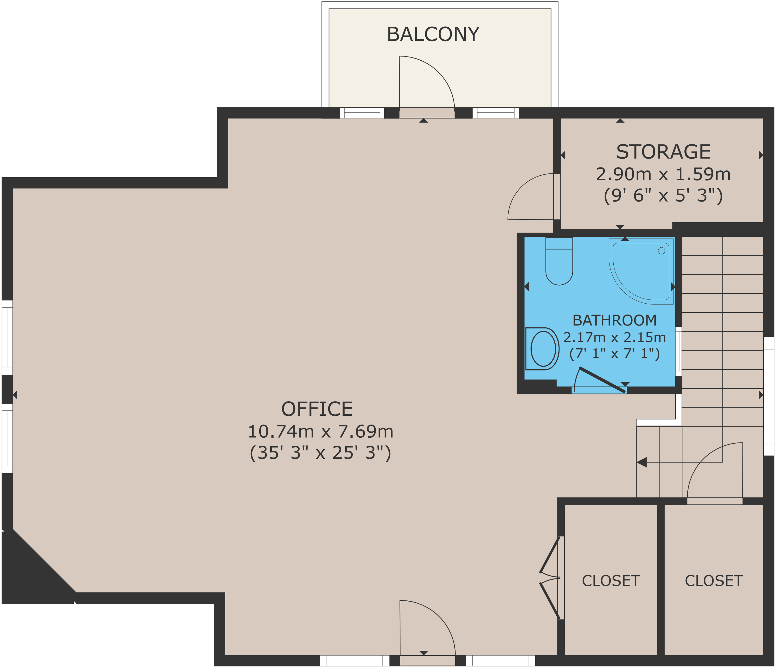
UPPER FLOOR
