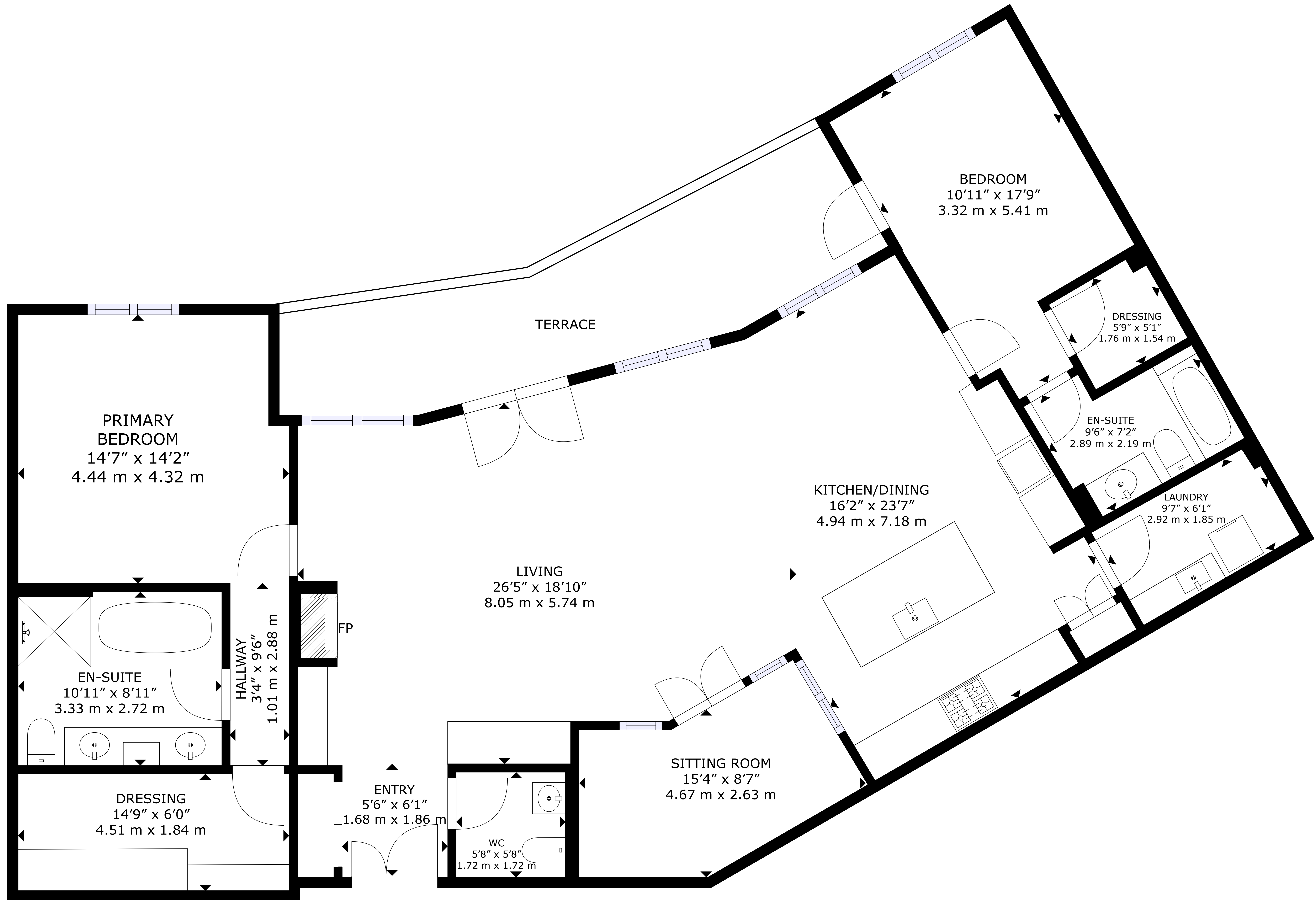
FLOOR PLAN
