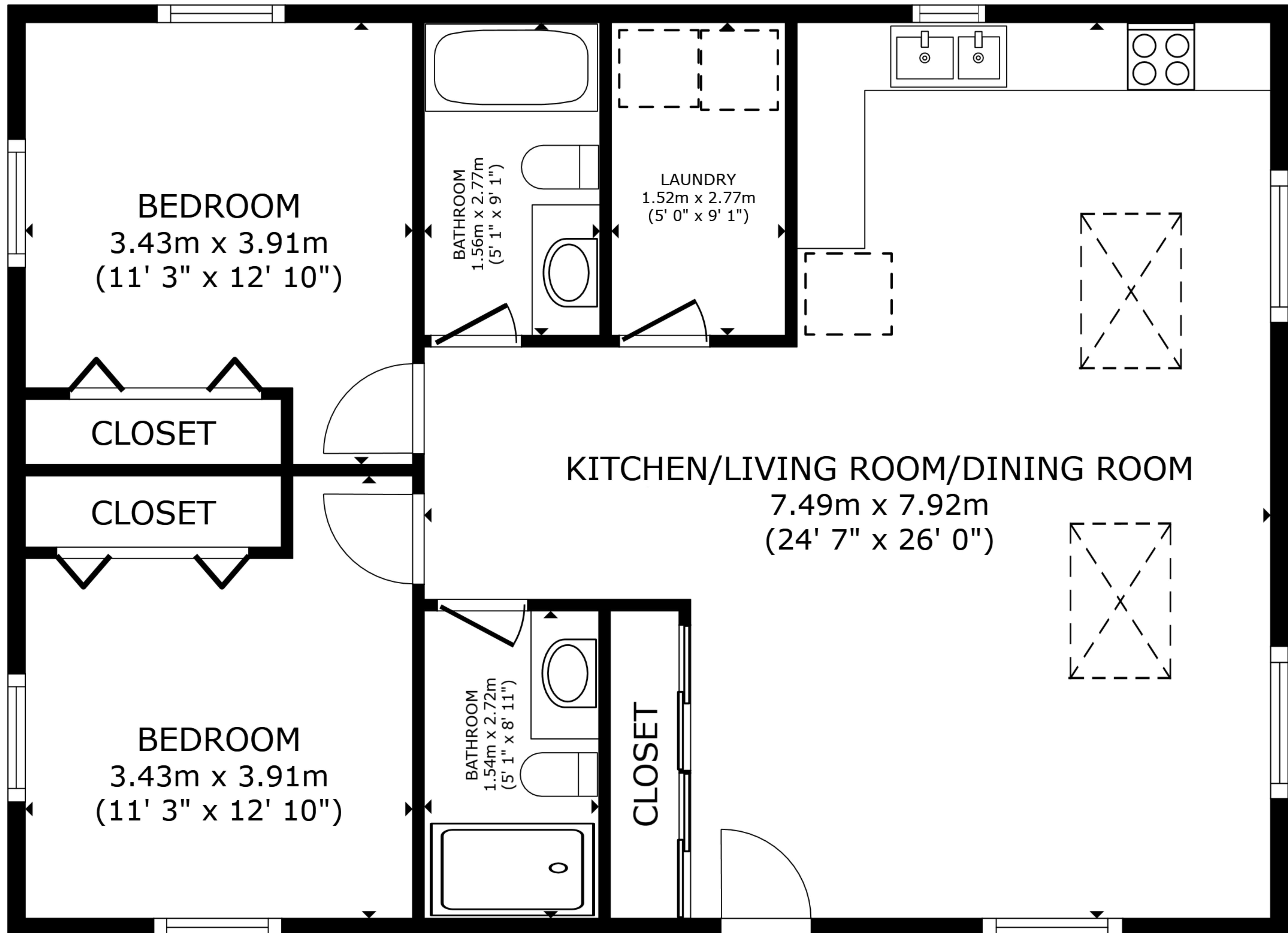
FLOOR PLAN
