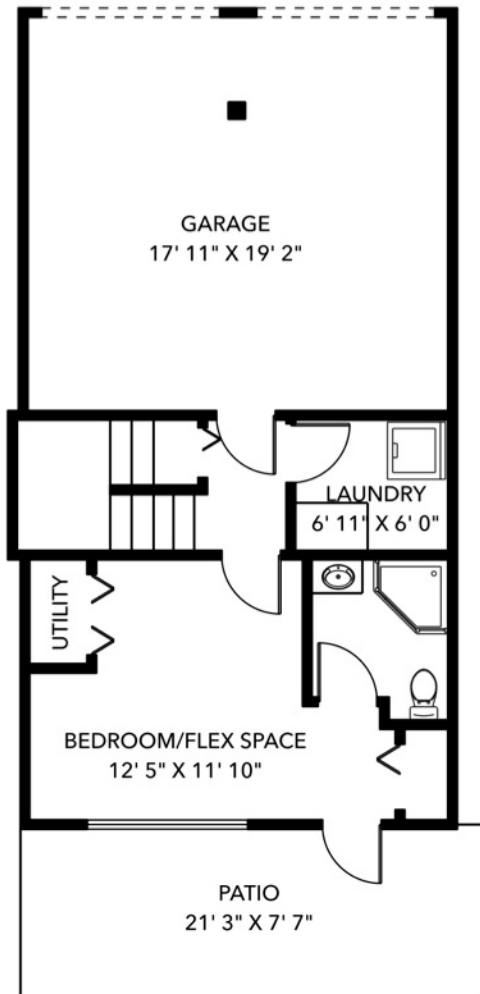
LOWER LEVEL 372 SQ.FT. CH: 8'0"
