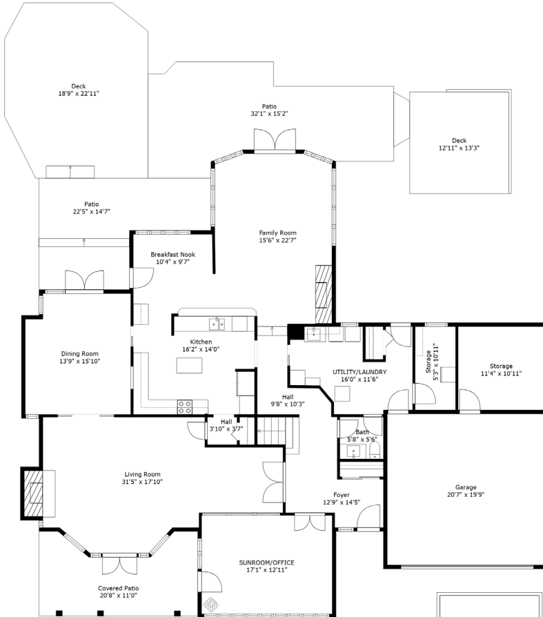
Floor 1
