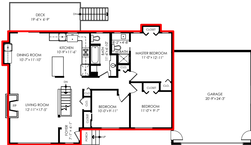
Main Floor Plan Floor Area: 1261 sq.ft. Ceiling Height: 7'-11"
