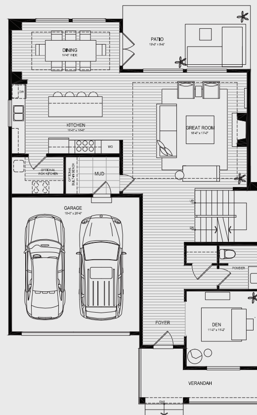
Main - 1,270 sq. ft.
