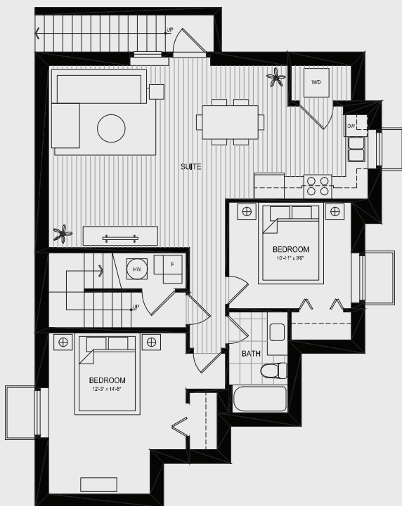
Lower with optional legal suite - 1,073 sq. ft.
