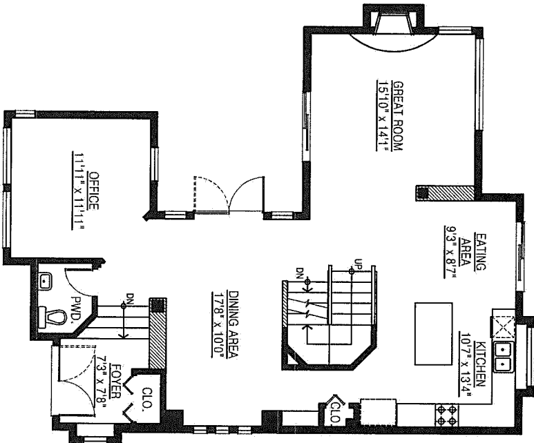
MAIN FLOOR PLAN FLOOR AREA: 1,147 sq.ft.
