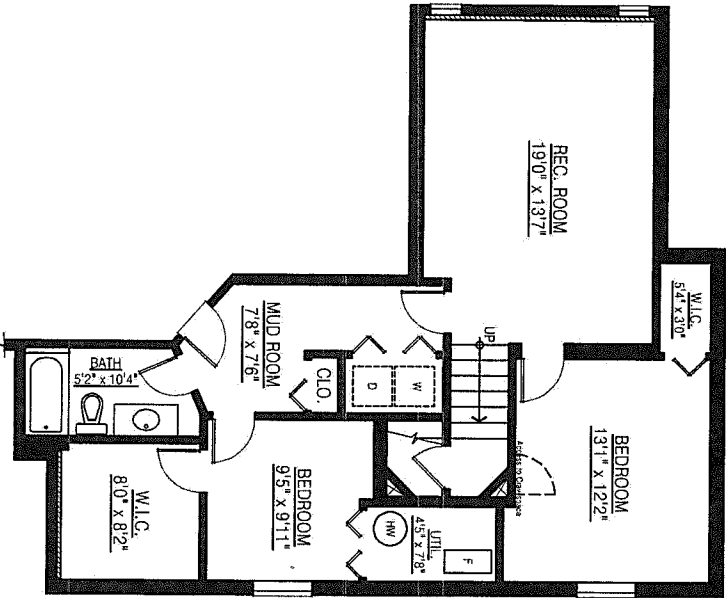
BASEMENT FLOOR PLAN FLOOR AREA: 978 sq.ft.
