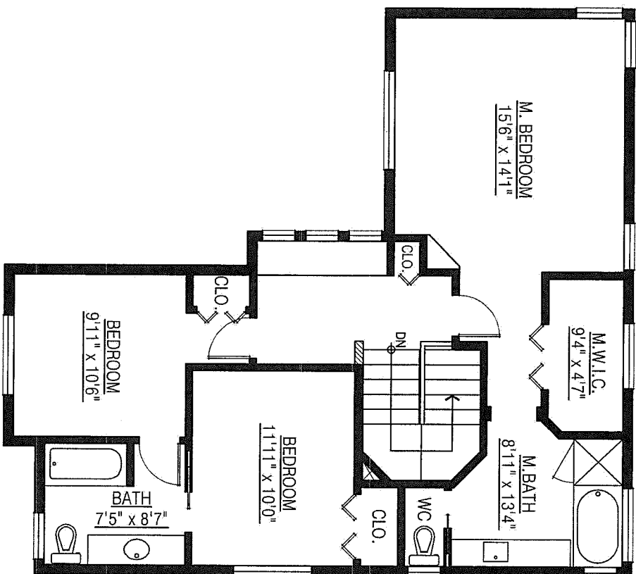
UPPER FLOOR PLAN FLOOR AREA: 900 sq.ft.
