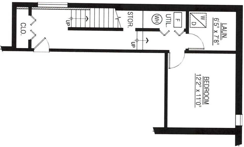
BASEMENT FLOOR PLAN FLOOR AREA: 425 sq.ft.
