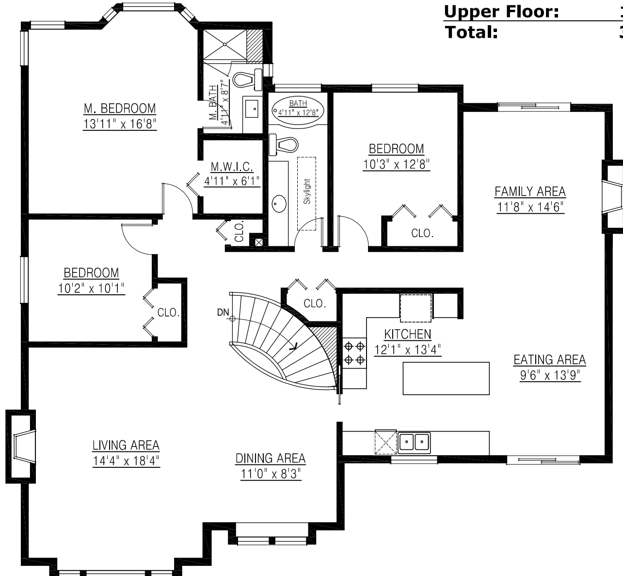
UPPER FLOOR PLAN FLOOR AREA: 1,761 sq.ft.
