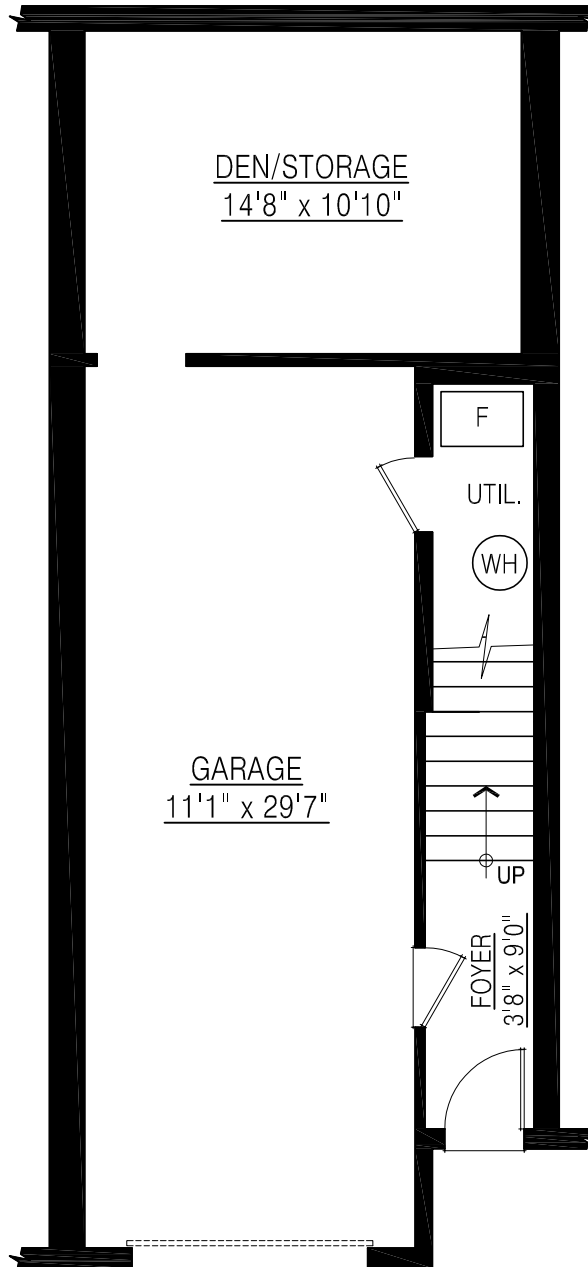
LOWER FLOOR PLAN FLOOR AREA: 308 sq.ft.
