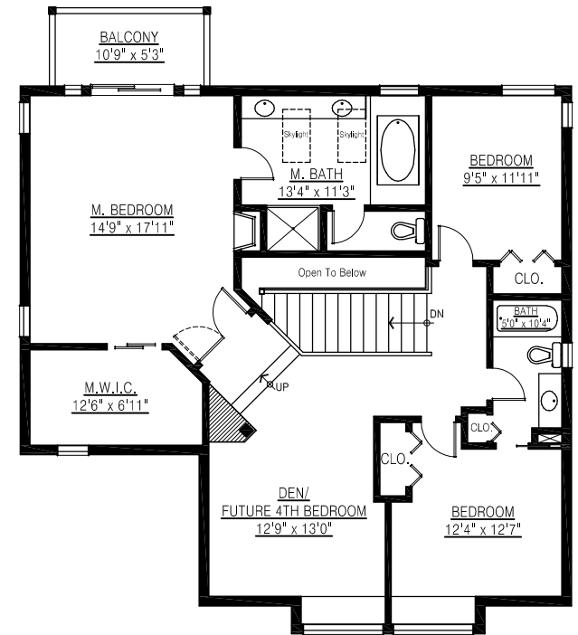
UPPER FLOOR PLAN FLOOR AREA: 1,268 sq.ft.
