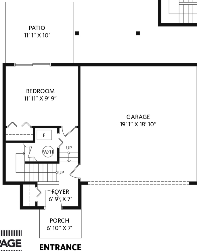
Lower Floor - 288 sq.ft. Ceiling height - 8' 0"
