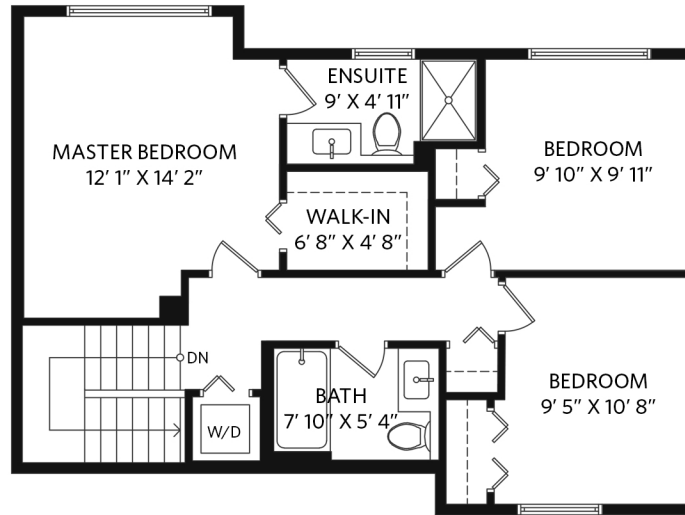
Upper Floor - 693 sq.ft. Ceiling height - 8' 0"
