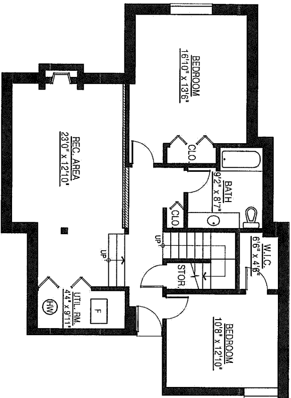
BASEMENT FLOOR PLAN FLOOR AREA: 1,095 sq.ft.
