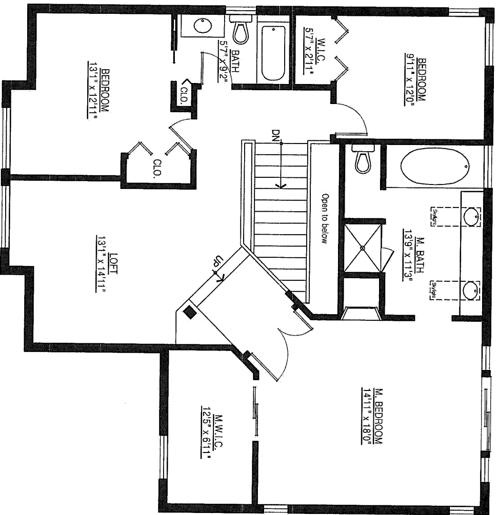
UPPER FLOOR PLAN FLOOR AREA: 1,334 sq.ft.
