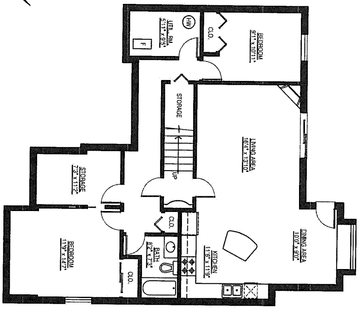
LOWER FLOOR PLAN FLOOR AREA: 1,303 sq.ft.
