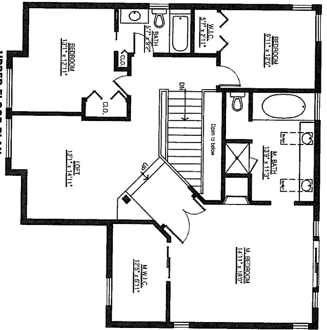
UPPER FLOOR PLAN FLOOR AREA: 1,334 sq.ft.
