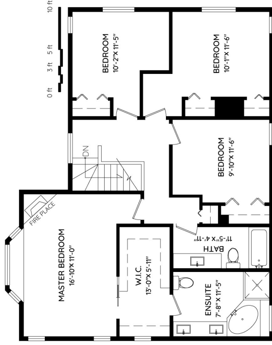
UPPER FLOOR 1,071 SQ.FT. CH: 9'-0"
