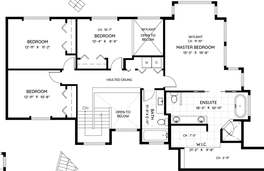
UPPER FLOOR 1,434 SQ.FT. CH: 11'-3" (Vaulted C.H.)
