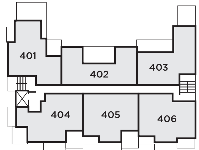
FOURTH FLOOR
