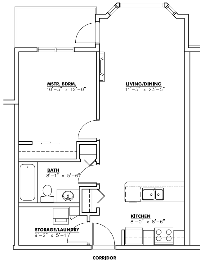
UNIT TYPE 'E' 672 sf
