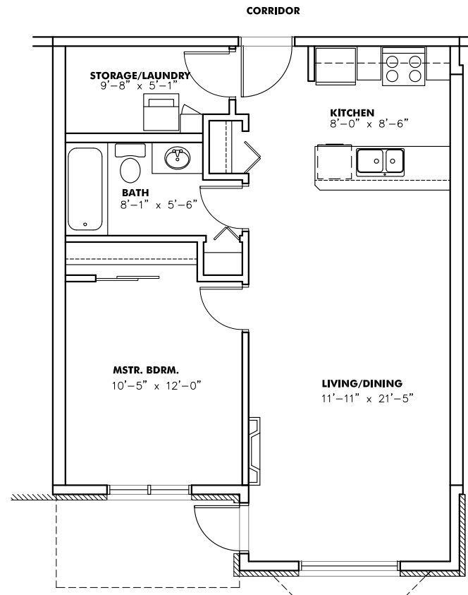
UNIT TYPE 'C' 678 sf
