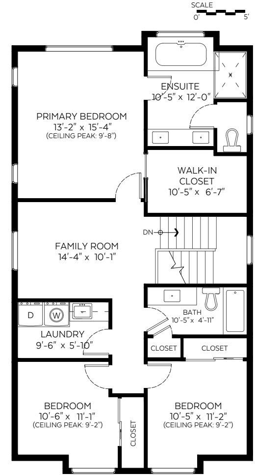
Upper Floor Plan Floor Area: 1,112 sq.ft. Ceiling Height: 8 ft.
