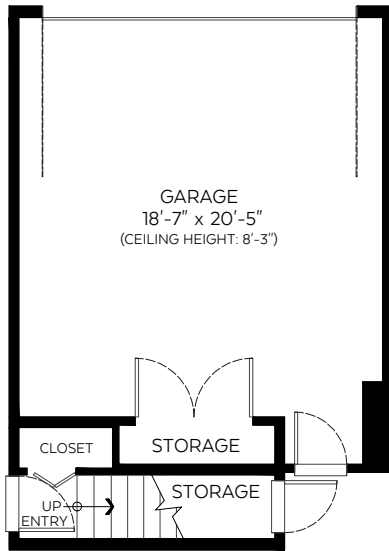
Suite Entry Floor Plan Floor Area: 75 sq.ft. Ceiling Height: 8 ft.
