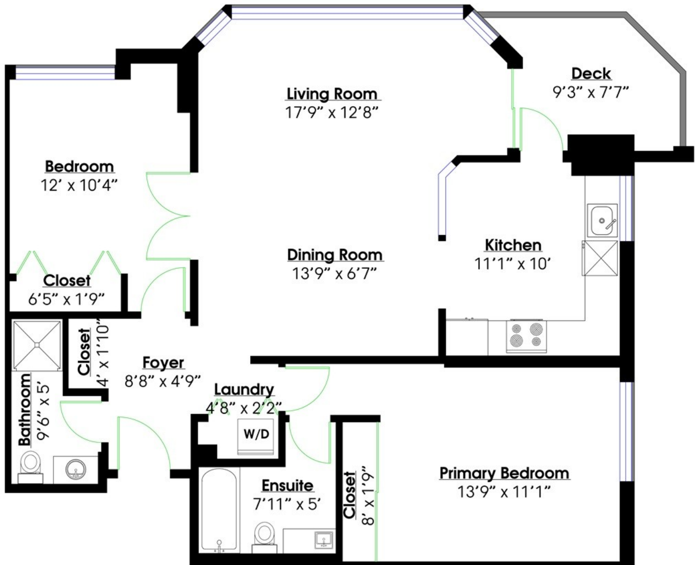
MAIN LEVEL Floor Area: 1,019 Sq. Ft. Ceiling Height: 8'
