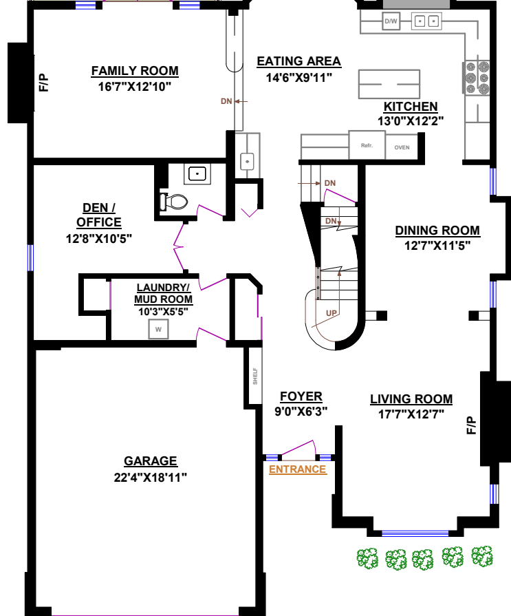
MAIN FLOOR
