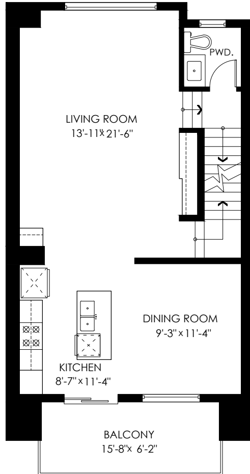
First Floor Plan Floor Area: 722 sq.ft. Ceiling Height: 9'
