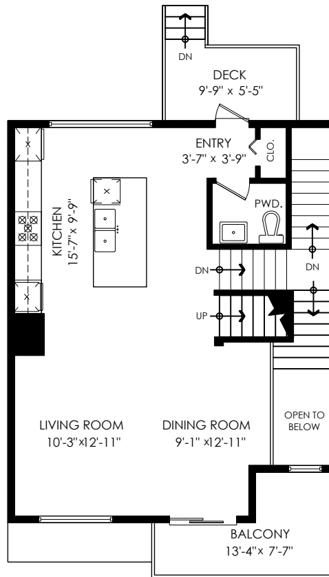
Main Floor Plan Floor Area: 677 sq.ft. Ceiling Height: 8'-11"
