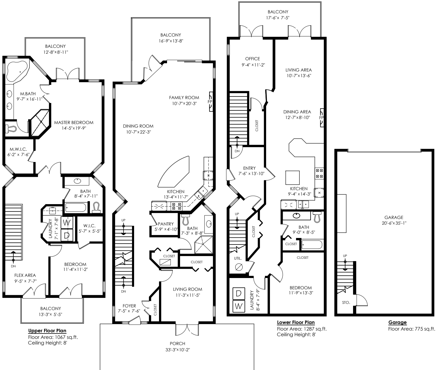
Main Floor Plan Floor Area: 1209 sq.ft. Ceiling Height: 8'-10"
