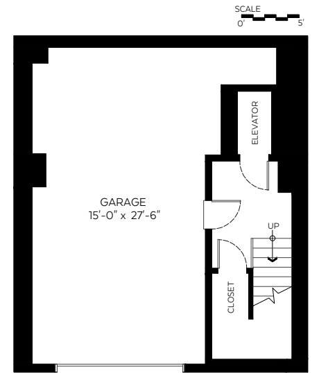
Basement Floor Plan Floor Area: 213 sq.ft.
