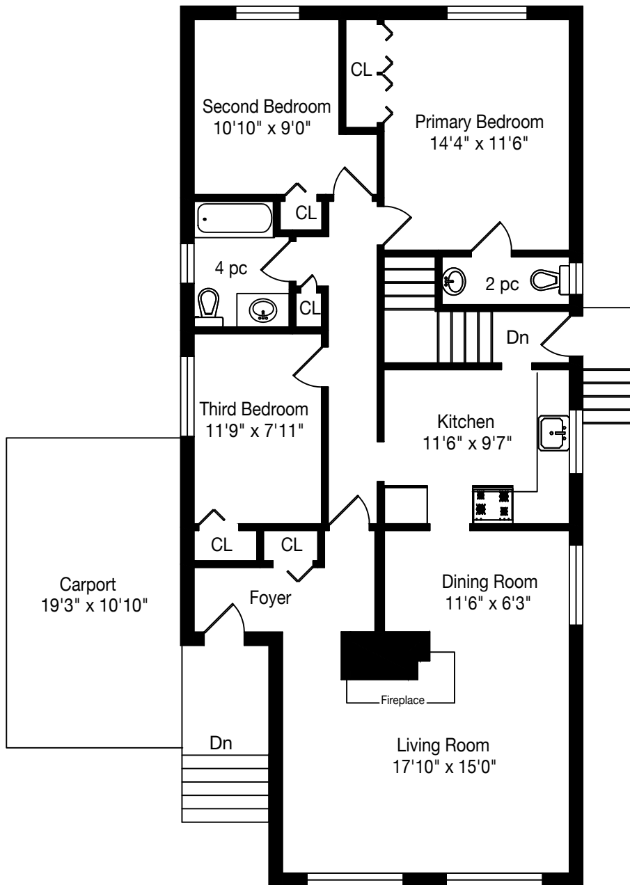
Main Floor
