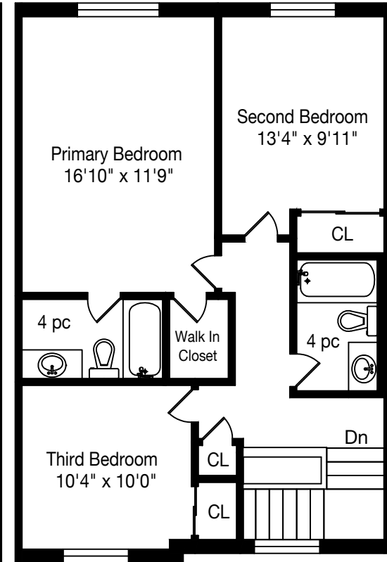
Second Floor 775 Square Feet
