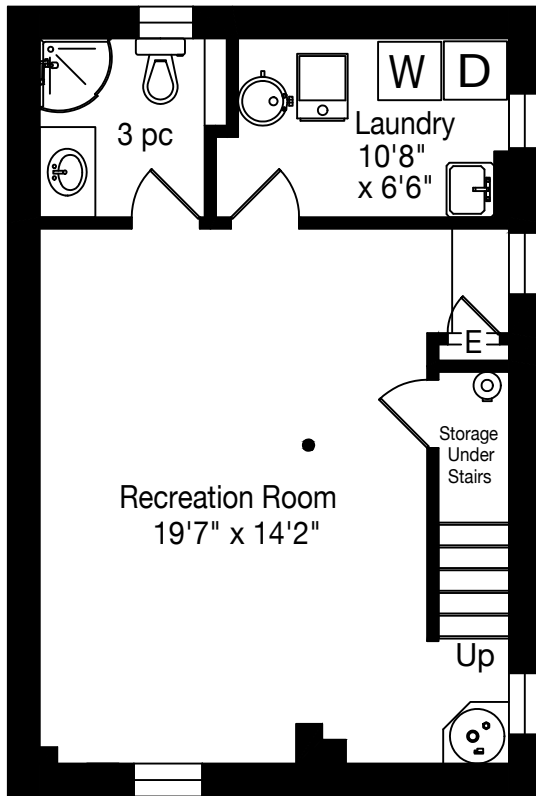
Lower Level
