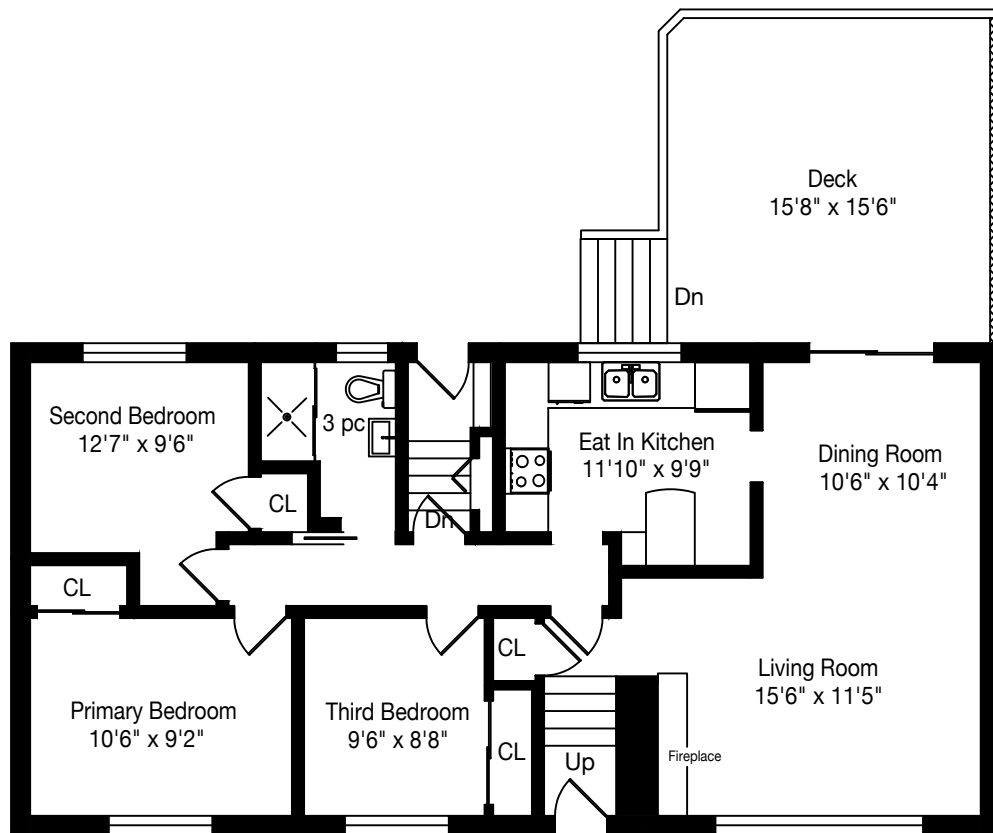
Main Floor 1123 Square Feet
