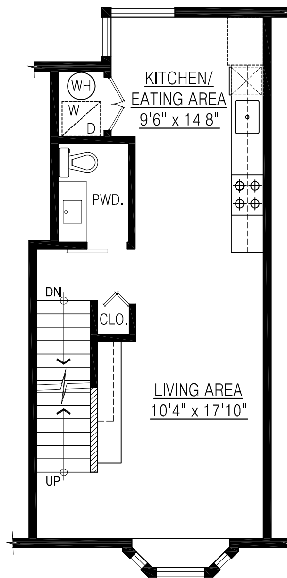
MAIN FLOOR PLAN FLOOR AREA: 463 sq.ft.
