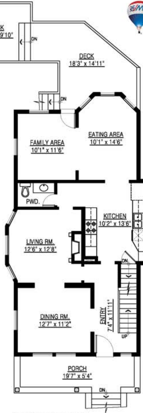
MAIN FLOOR PLAN FLOOR AREA: 971 sq.ft.
