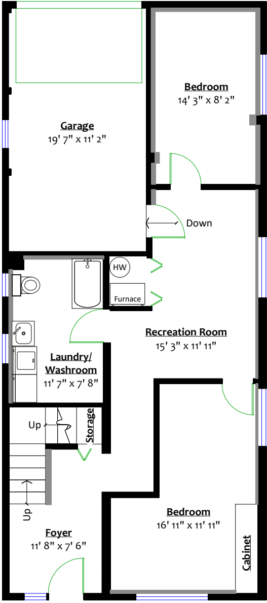
LOWER LEVEL Floor Area: 791 Sq. Ft. Ceiling Height: 8'
