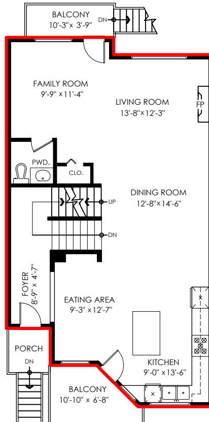
Main Floor Plan Floor Area: 947 sq.ft. Ceiling Height: 9'
