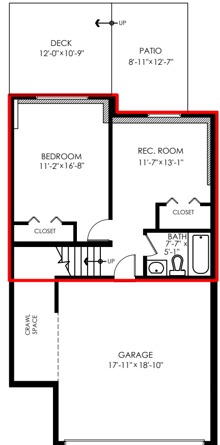
Lower Floor Plan Floor Area: 505 sq.ft. Ceiling Height: 7'-11"
