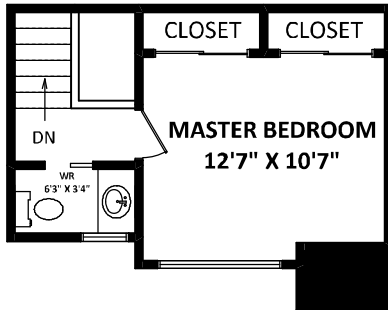
TOP FLOOR: 240 SQ.FT.
