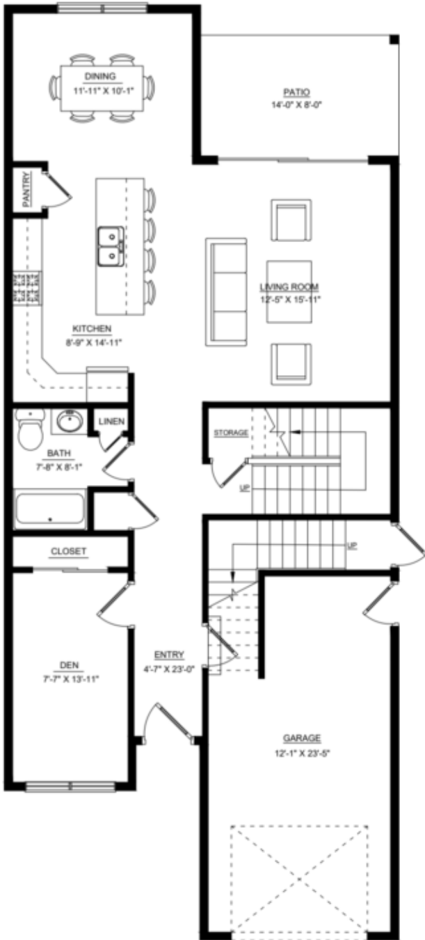
CEDAR PLAN MAIN FLOOR
