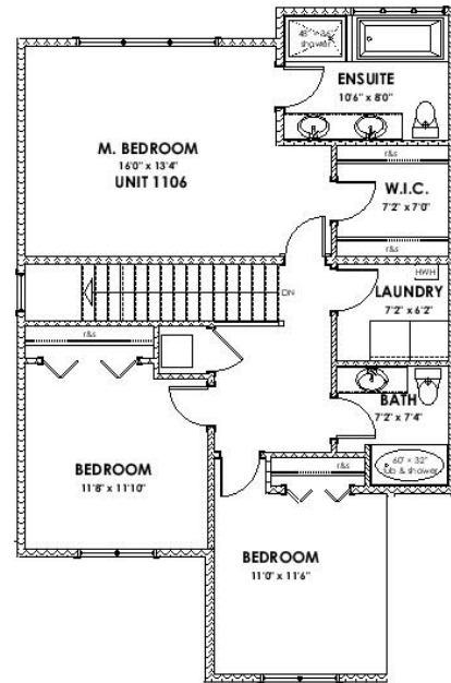
UPPER FLOOR 963 SQ FT
