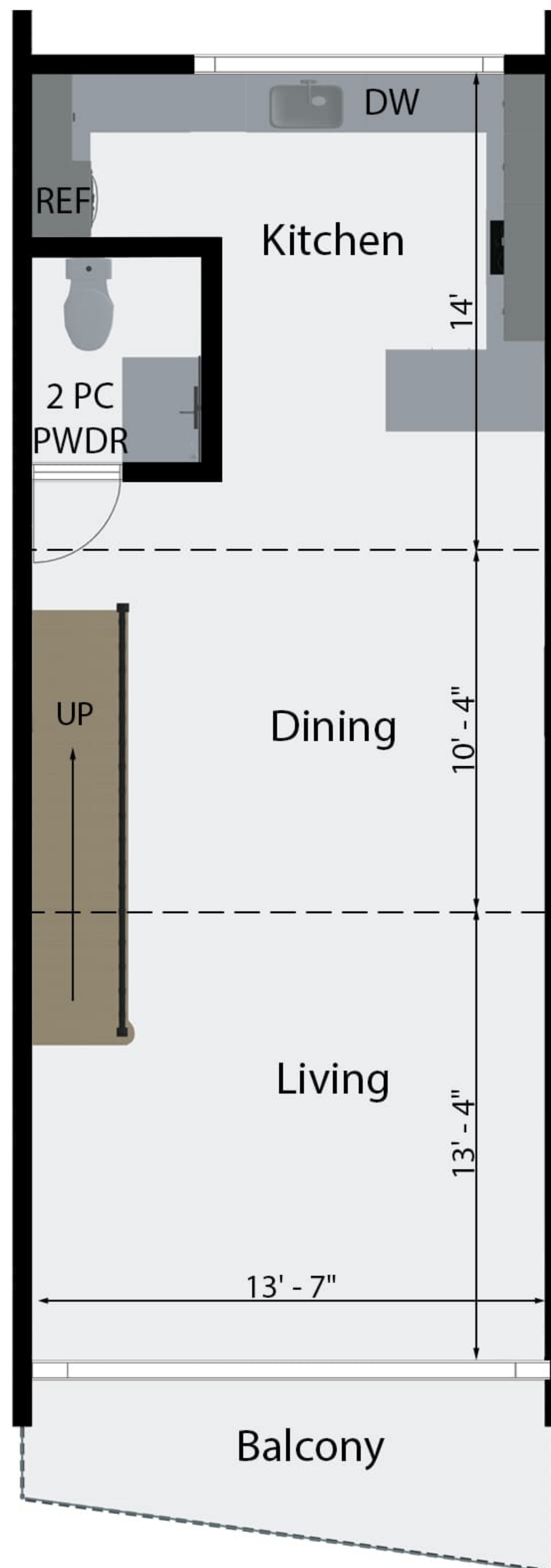
SECOND FLOOR 480 SQ.FT. 9' CEILING HEIGHT
