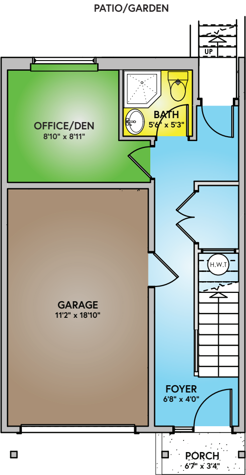
LOWER FLOOR (559 sq. ft.)
