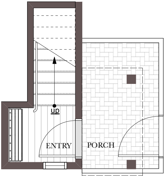
Main Floor Plan: Building 7
