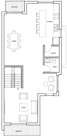
LEVEL 2 - 819 SF DECKS - 81 SF
