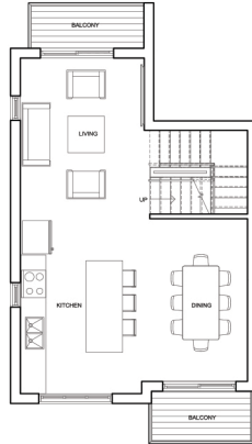
LEVEL 2 - 512 SF DECKS - 72 SF
