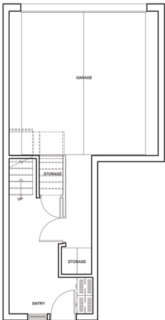
LEVEL 1 - 235 SF (LEVEL 1 + GARAGE) - 612 SF
