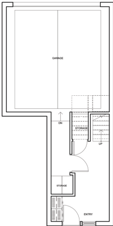
LEVEL 1 - 239 SF (LEVEL 1 + GARAGE) - 636 SF
