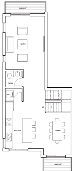
LEVEL 2 - 670 SF DECKS - 78 SF
