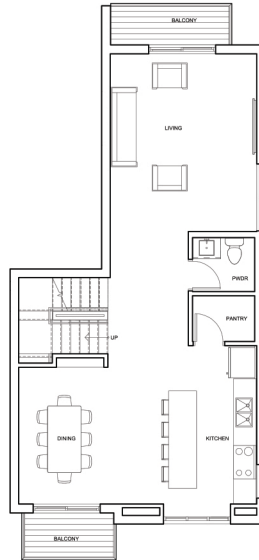
LEVEL 2 - 702 SF DECKS - 68 SF
