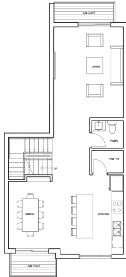
LEVEL 2 - 669 SF DECKS - 70 SF
