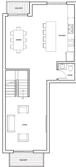
LEVEL 2 - 688 SF DECKS - 62 SF
