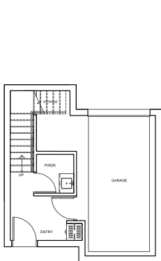
LEVEL 1 - 186 SF (LEVEL 1 + GARAGE) - 397 SF
