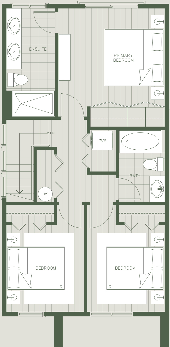
UPPER LEVEL
