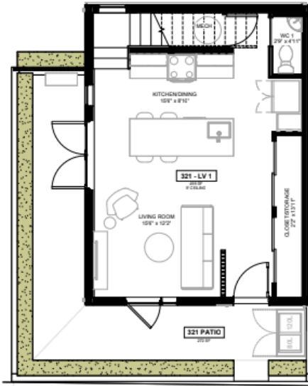
1 Marketing Plans - Unit 321 LVL 1 - 499 sq ft A.220M 1:50
