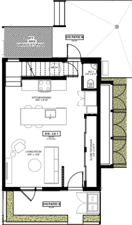
4 Marketing Plans - Unit 315 LVL 1 - 490 sq ft A.221M 1:50
