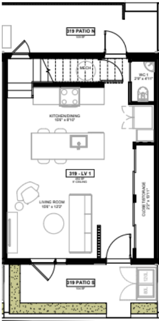
4 Marketing Plans - Unit 319 LVL 1 - 492 sq ft A.220M 1:50
