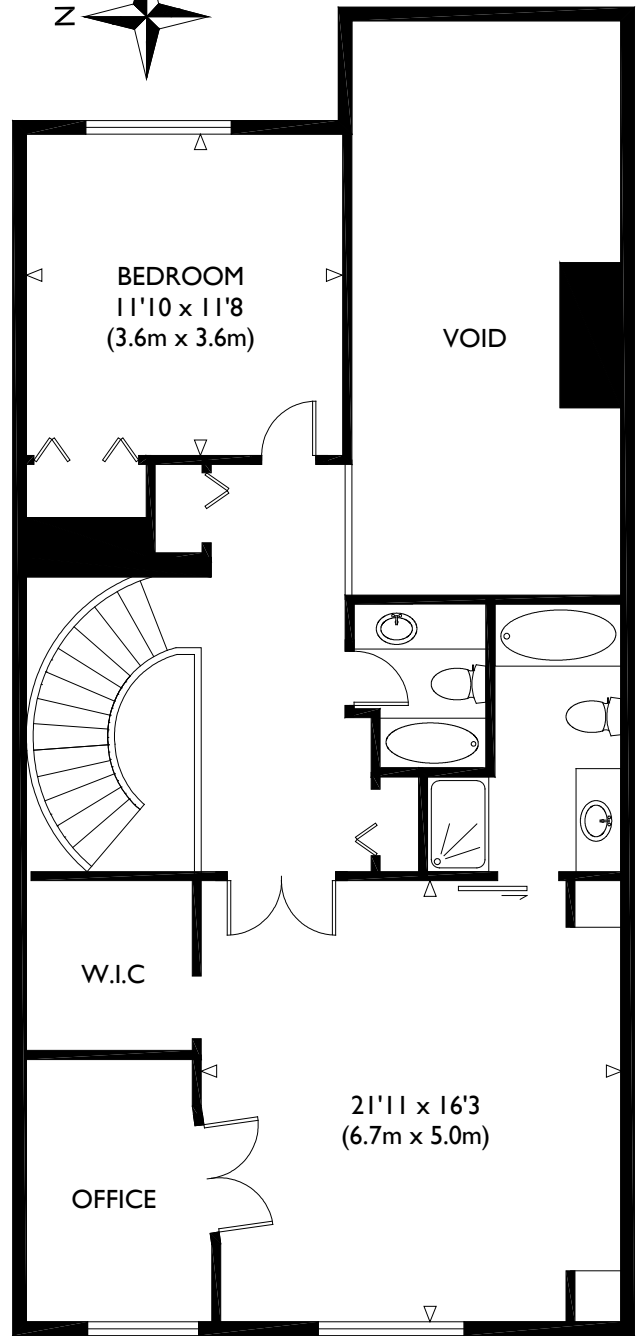
UPPER FLOOR GROSS INTERNAL FLOOR AREA 940 SQ FT
