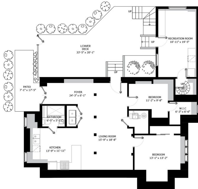
LOWER FLOOR PLAN Ceiling Height: 7'-0"
