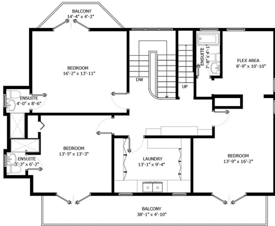
UPPER FLOOR PLAN Ceiling Height: 9'-0"
