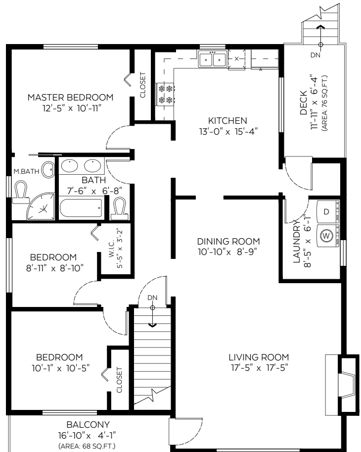
Main Floor Plan Floor Area: 1,381 sq.ft.
